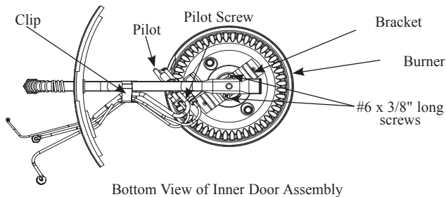
Bottom View of Inner Door Assembly
