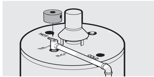
Typical Top Connect T & P Arrangement.
